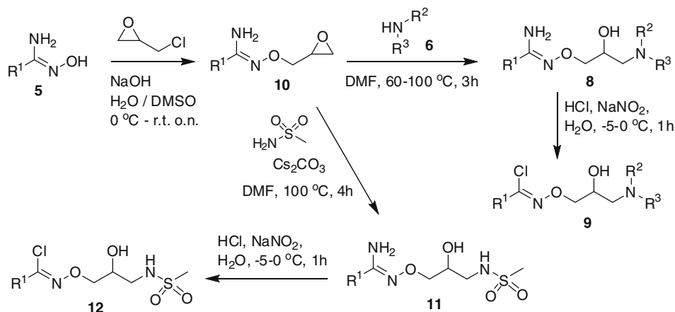
Scheme 2. Synthetic method B for chloro-oxime derivative preparation.
